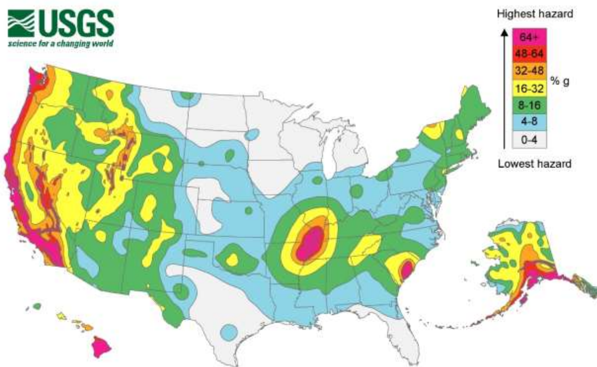
Figure 3-3 U.S. Geological Survey 2008 Hazard Map
