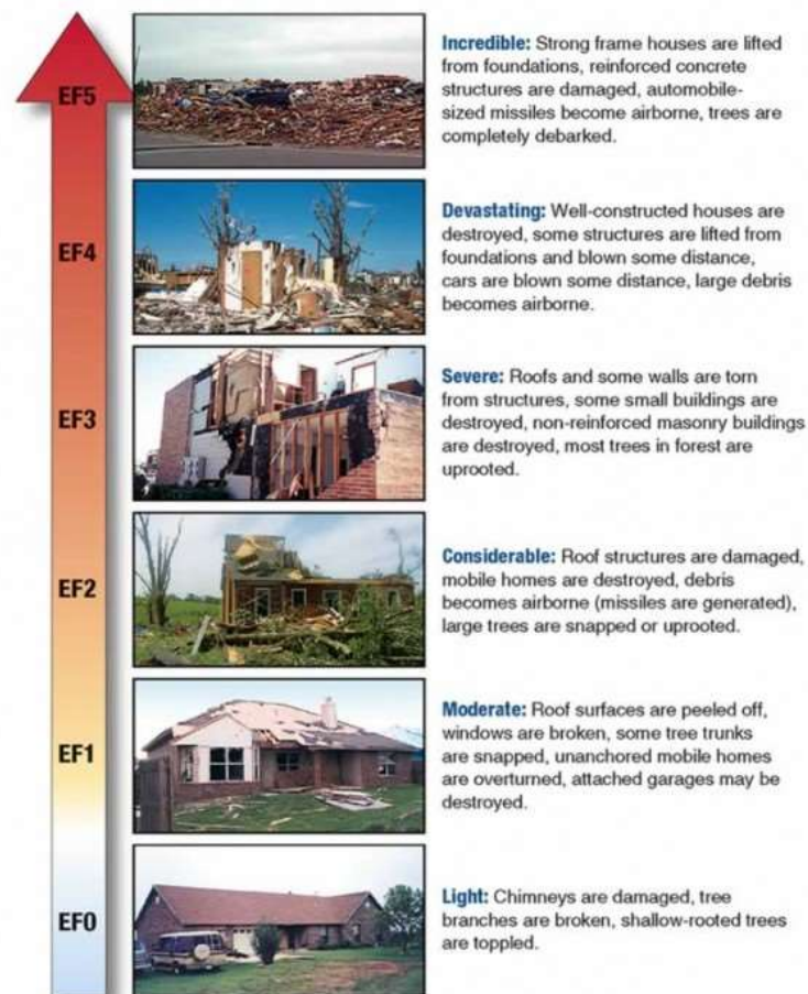
Figure 3-11 Tornado Destruction based on Enhanced Fujita
