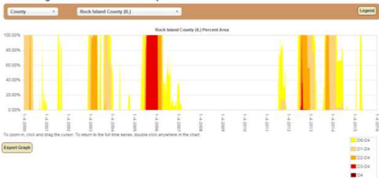
Figure 3-1 U.S. Drought Monitor
