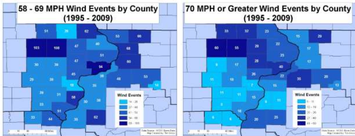
Figure 3-8 Wind Events by County
