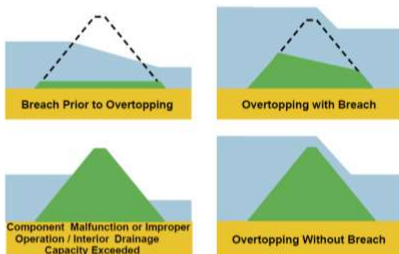
Figure 3-4 Levee Breach Diagram
