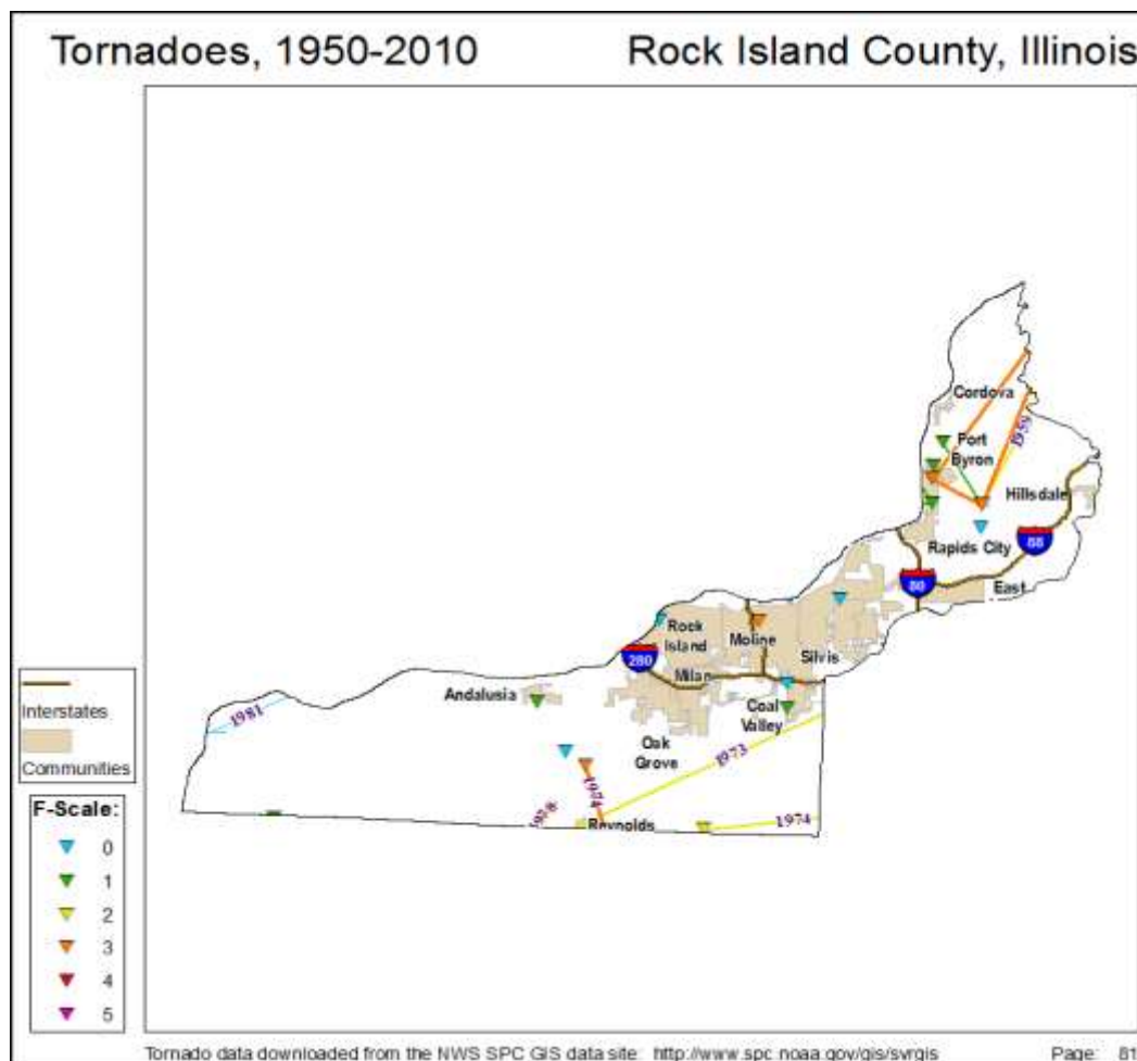
Figure 3-9 Historic Tornado Touchdowns by Severity in Rock Island County
